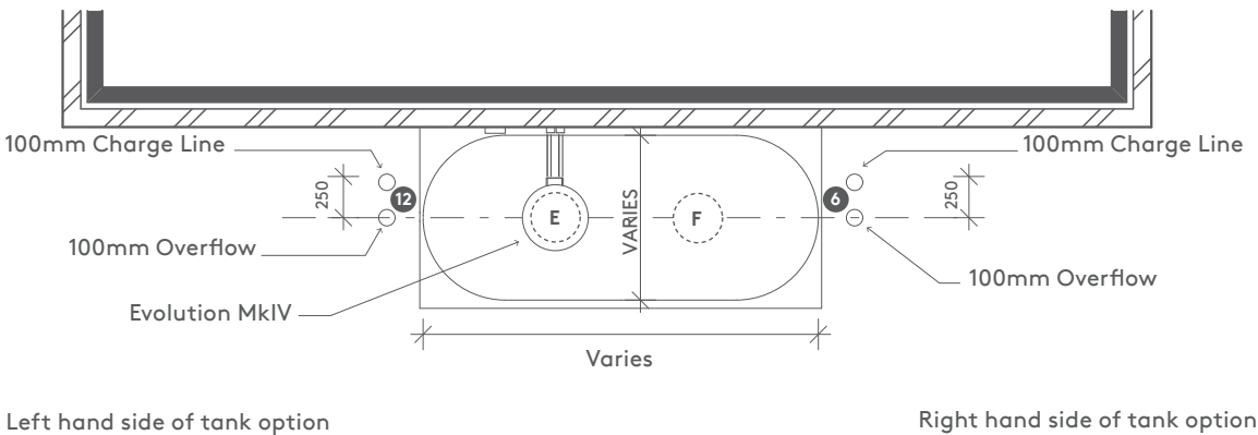
PLAN VIEW TYPICAL
