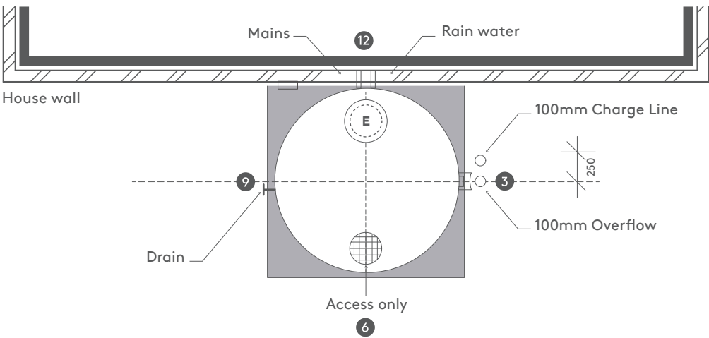
PLAN VIEW TYPICAL
